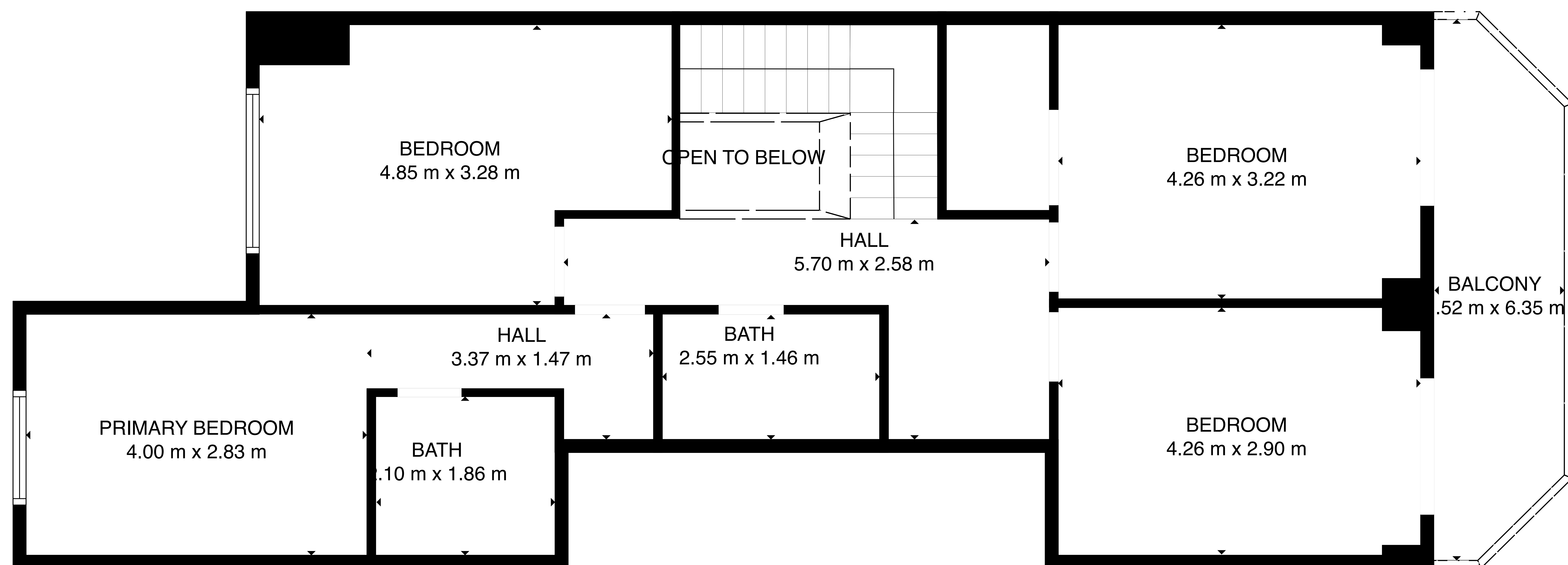
FLOOR 2
